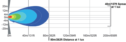
MIL-RXP1260T / 4009998 60° BEAM PATTERN
